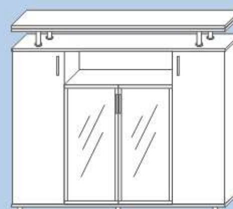
2.15.2 KOMODA 1600x380x1330
