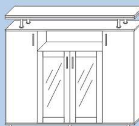
2.15.1 KOMODA 1600x380x1330
